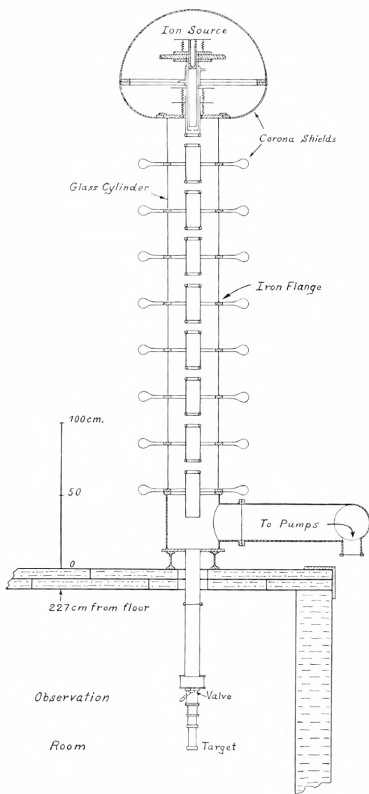
Fig. 12. Construction of acceleration tube with extension into observation room.
