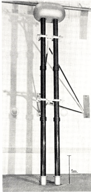
Fig. 5. Voltmeter resistance. The left column serves as mechanical support and as a part of the oil circulation system.
