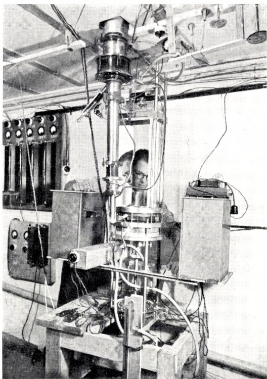
Fig. 17. Target tube and cloud chamber.
