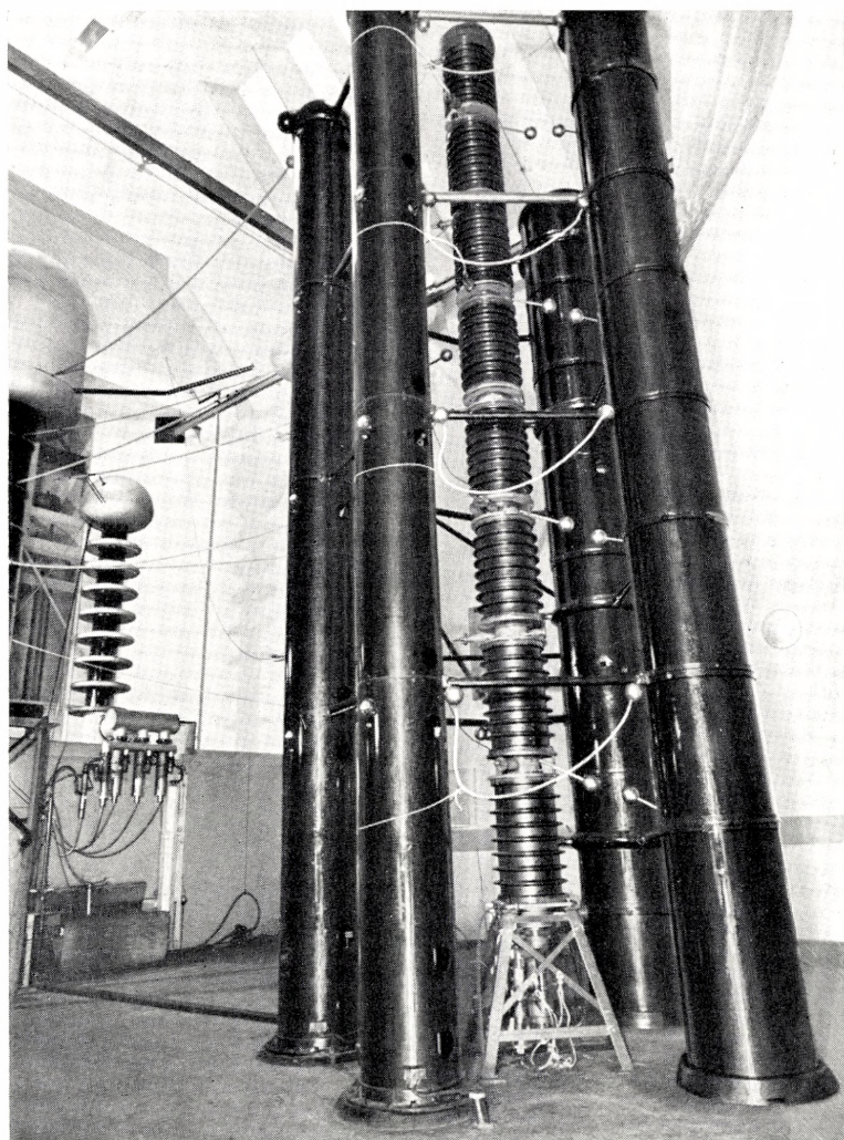
Fig. 9. View from south-west corner of the hall showing generator with rectifier column, spark gaps and protective resistances (photographically distorted).
