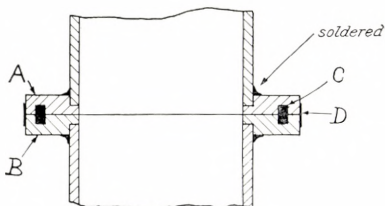
Fig. 15. Standard vacuum connection. A, B flanges held in position by the automobile piston ring C and made tight by a rubber band D and glyptal lacquer.
