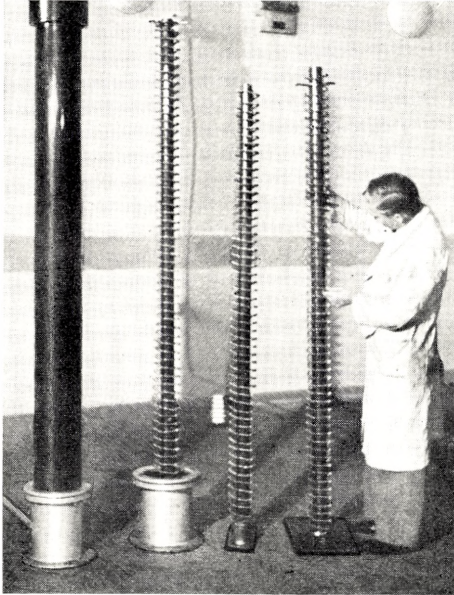
Fig. 4. Voltmeter resistance before assembly.
