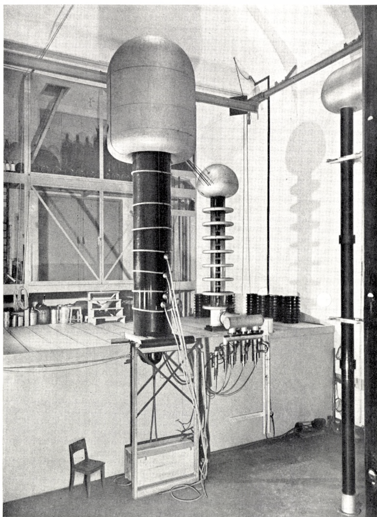
Fig. 10. Acceleration tube and power stack mounted on top of the observation room. To the extreme right is seen the high tension resistance and a part of the generator.
