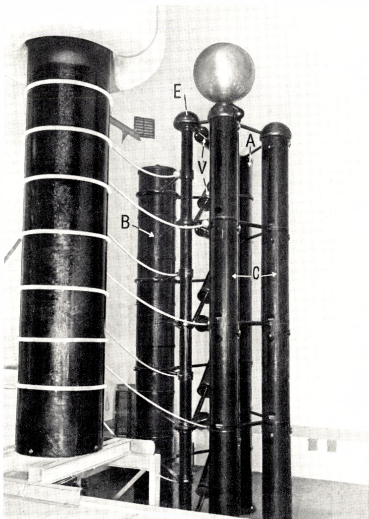
Fig. 3 a. View of generator set seen from the roof of the observation room. A: high tension transformers. B: feeding transformers. C: Generator columns for filament current. E: condenser column. V: rectifier tubes.
