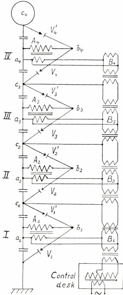
Fig. 2. Electrical circuit of the generator showing the four Greinacher sections I—IV mounted one on top of the other. A_n : High tension transformers. B_n : Feeding transformers. V_n : Rectifier tubes.
