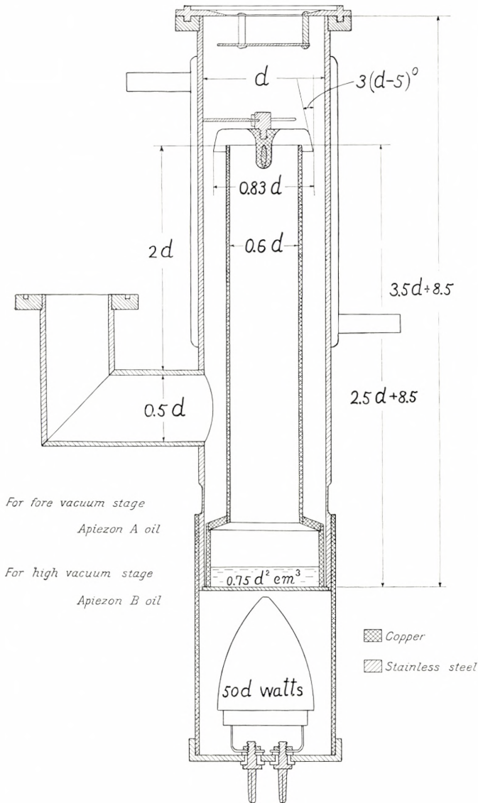
Fig. 13. Vacuum pump details. The dimensions of the pump, the amount of oil to be used and the heating power are given as functions of the diameter d of the envelope in cm.
