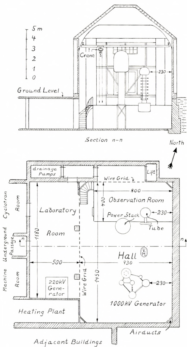
Fig. 1. Plan of building with high tension hall and adjoining laboratories, indicating also the position of the high tension equipment.
