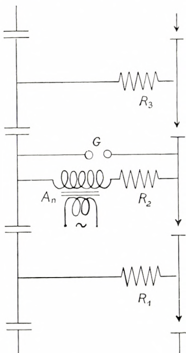
Fig. 7. Diagram of one stage of the modified circuit of the generator with the resistances R_1 , R_2 , R_3 and the spark gap G in order to protect the high tension transformer A_n .
