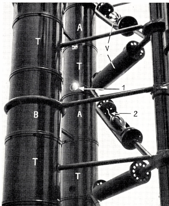
Fig. 8. Photograph of discharge between two high tension transformers (arrow 1) and along a rectifier tube (arrow 2). The figure shows the arrangement of the rectifier tubes and the columns with the high tension transformers (A) and feeding transformers (B) separated by supporting tubes (T).
