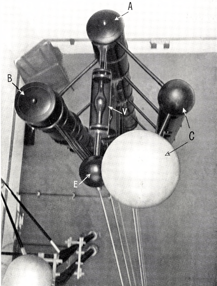
Fig. 3 b. View of generator seen from the roof of the hall. A : high tension transformers. B : feeding transformers. C : Generator columns for filament current. E : condenser column. V : rectifier tubes. See also Fig. 8.
