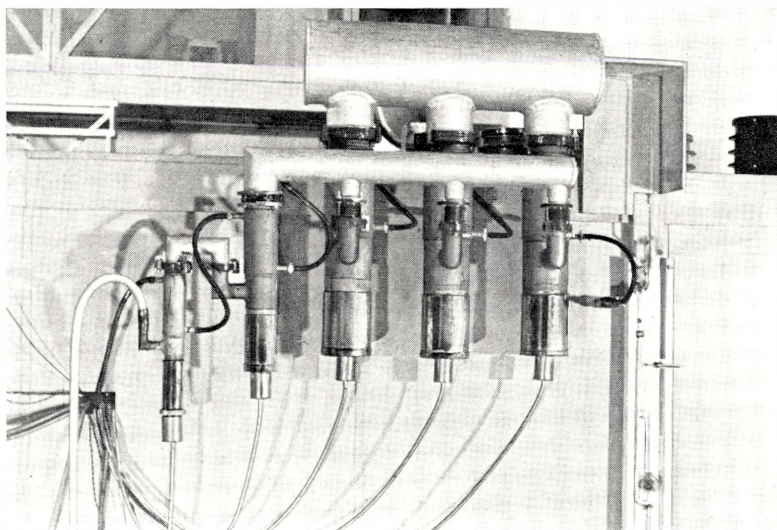
Fig. 14. Vacuum pump system used in connection with the acceleration tube consisting of three 5" pumps in parallel backed by a 3" and a 2" diffusion pump and a mechanical stage (not shown).
