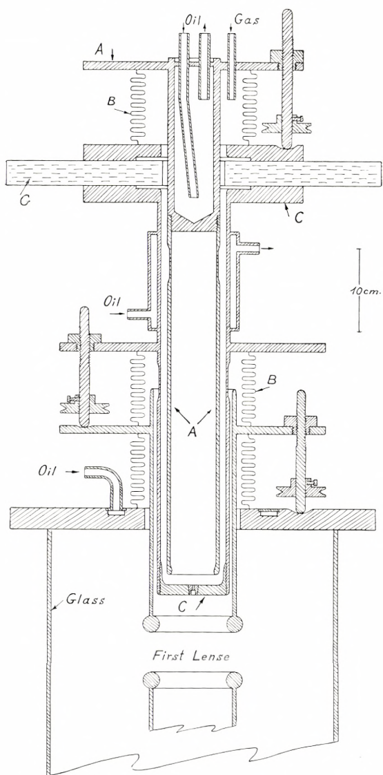
Fig. 11. High tension ion source. A: anode, C: cathode, B: vacuum tight bellows. G: glass insulator,
