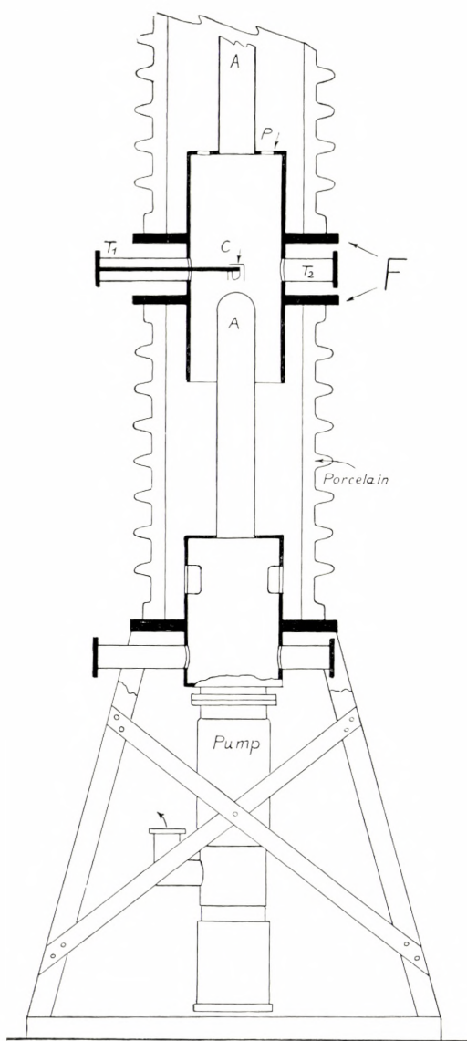
Fig. 6. First stage of rectifier column connected with a 5" oil diffusion pump. F : Flange separating the different sections. P : Perforated plate carrying anode. C : Cathode which can be removed through the tube T 1 .
